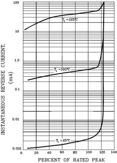
FIG.5-TYPICAL REVERSE CHARACTERISTICS
